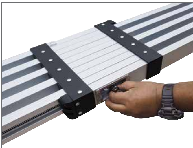
LOCKING MECHANISM TO FIX PLANK AT DESIRED LENGTH
