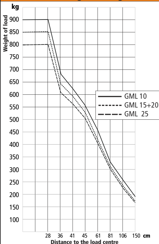
Safe working load diagram
